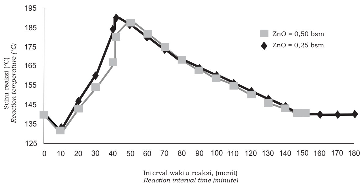
Gambar 2. Kenaikan suhu reaksi pada sintesis faktis coklat (15 kg minyak/ batch ) Figure 2. Increase of reaction temperature in brown factice synthesis (15 kgs of oil/ batch )
