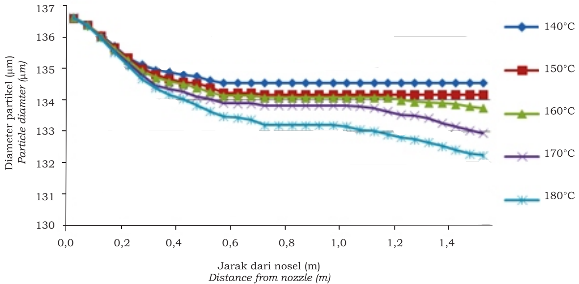
Gambar 8. Prediksi diameter partikel tepung lateks di ruang pengering pada berbagai suhu udara pengering dan kadar air lateks Figure 8. Diameter prediction of latex powder particle in the drying chamber at various drying air temperatures and latex water contents
