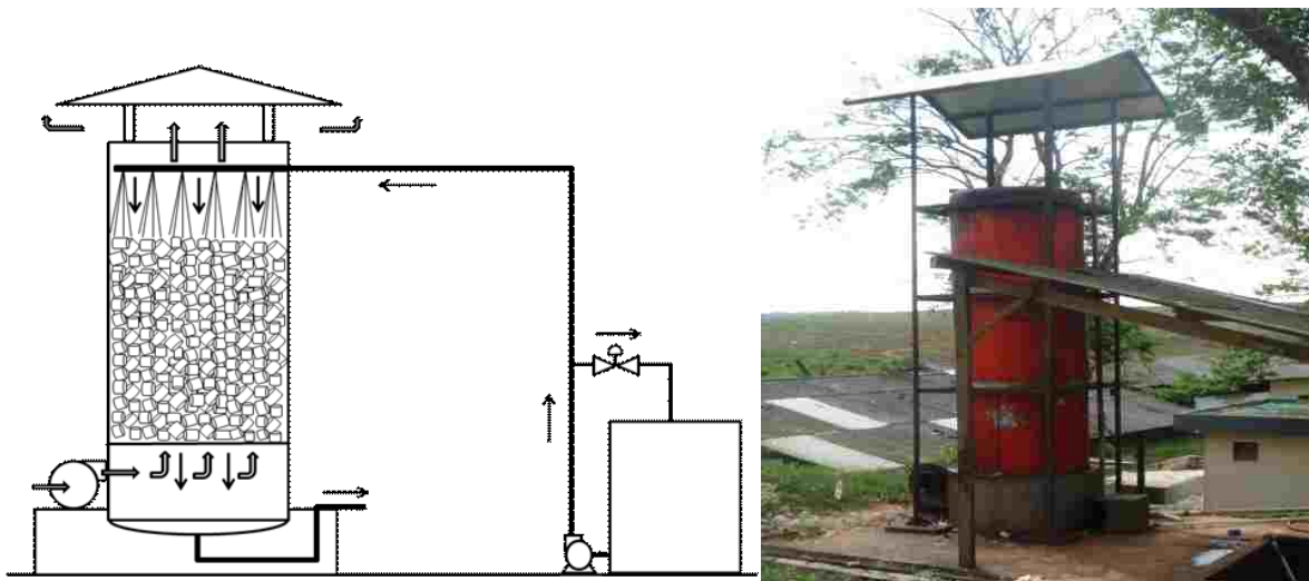
Gambar 3. Sketsa dan foto menara deammoniasi Figure 3. Sketch and picture of deammoniation tower
