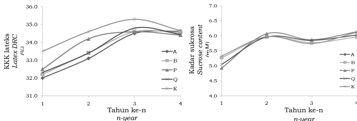
Gambar 2. a) Kadar karet kering lateks, dan b) kadar sukrosa pada pengujian EXPEX-315 Figure 2.a. Dry rubber content of latex, and b) sucrose content of EXPEX-315 trial
